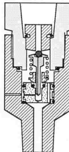
OUTLET 1/4" MPT
